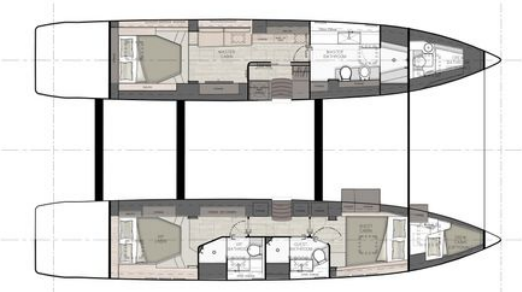
OMAYA 50 LAYOUT 3 CABIN HULLS
